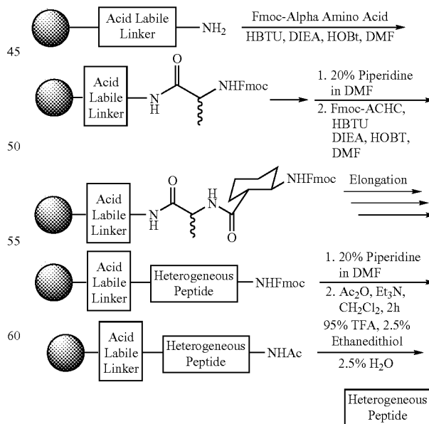
Scheme 3. Generalized Route for Solid Phase Synthesis
