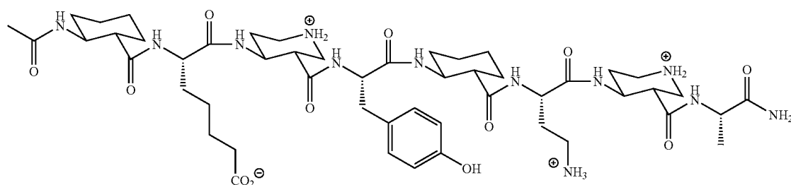
Ac-ACHC-E-PIP-Y-ACHC-K-PIP-A-NH 2 (SS) ACHC, (SS) PIP, (L) amino acids
