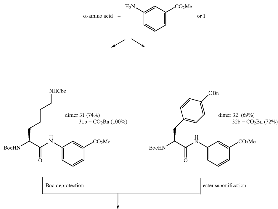
Scheme 11
