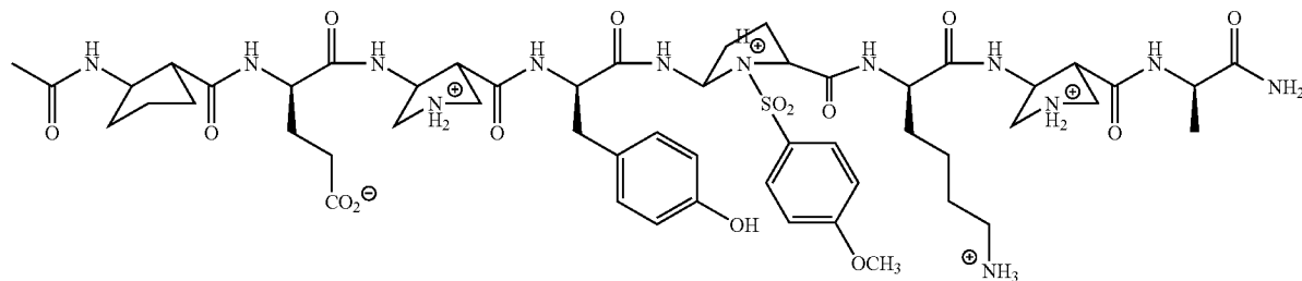
AC-ACPC-E-APC-Y-APC(SO 2 R)-K-APC-A-NH 2
