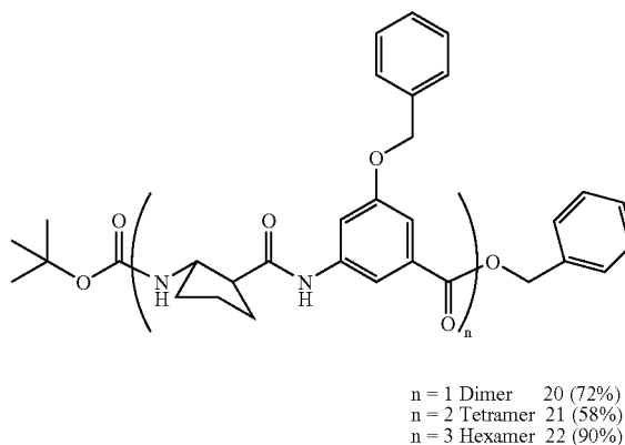
Scheme 8
