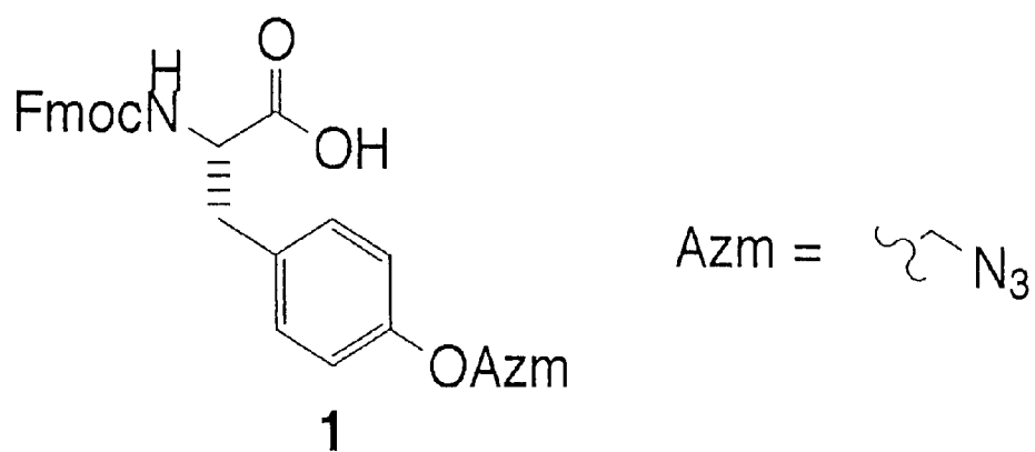
Figure 1. Target protected tyrosine building block
