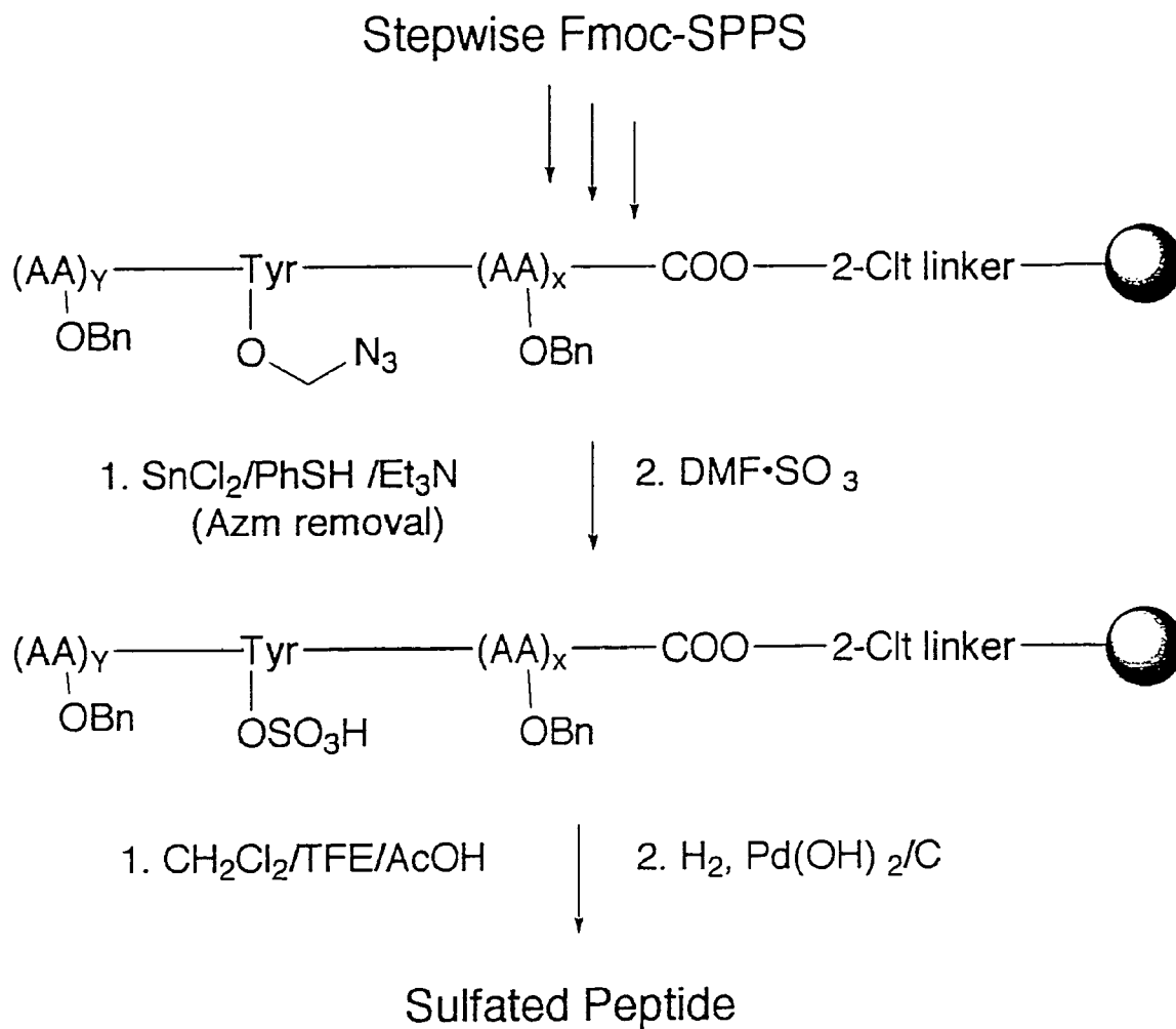
Figure 3. Overview of sulfated peptide synthesis.
