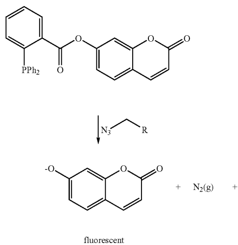
Scheme XV
