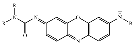
Scheme VIII
