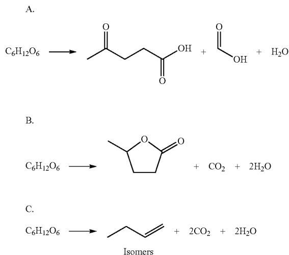
Scheme 2. Overall Balance of Sugar to Levulinic and Formic Acid (A), Sugar to GVL (B), and Sugar to Butene (C).
