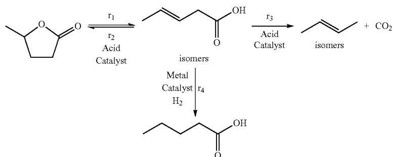
Scheme 3. Reactive pathway model
