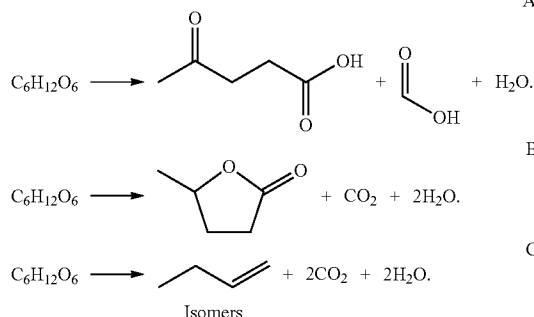
Scheme 2. Overall Balance of Sugar to Levulinic and Formic Acid (A), Sugar to GVL (B), and Sugar to Butene (C).
