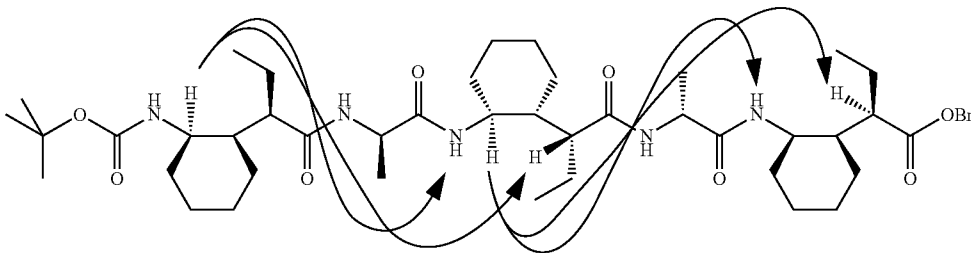
Scheme 1-7. Characteristic NOEs patterns observed for the 1:1 \alpha/\gamma -peptide hexamer in CDCl 3 .
