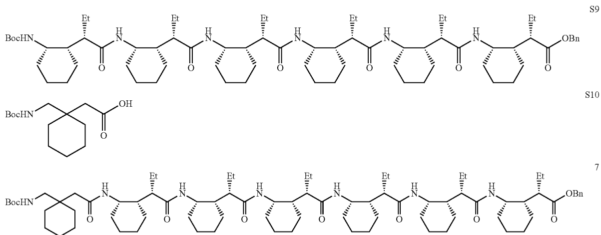
Scheme 7-3.
