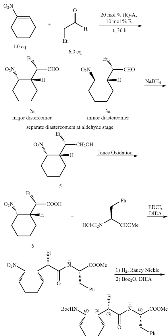
Scheme 1-1. Determination of d.r. of a Michael product by ^1H NMR assay
