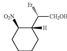
(S)-2-((1S,2R)-2-Nitrocyclohexyl)butan-1-ol 8
