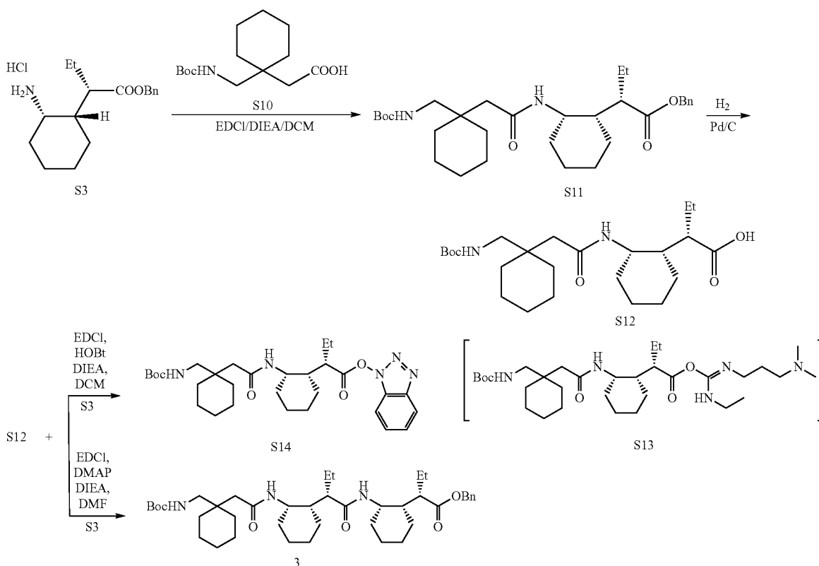
Scheme 7-4. Synthesis of oligomers S11 and 3.
