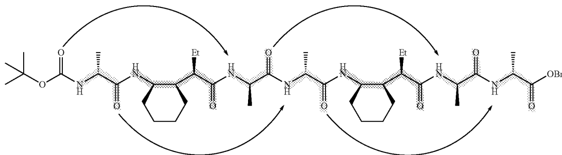
Scheme 8.3. An \gamma\alpha\alpha -peptide having four 12-membered ring hydrogen bonds.
