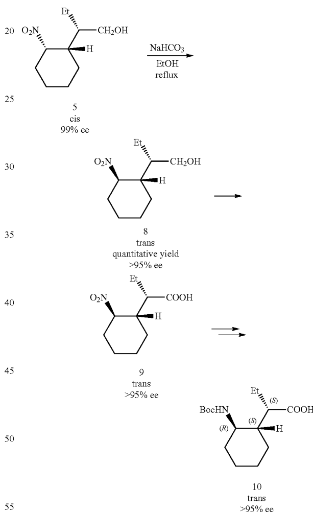
Scheme 1-6. Synthesis of cyclic γ-Amino Acid
