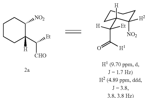
Scheme 1-2. 1 H NMR analysis of isolated product 2a
