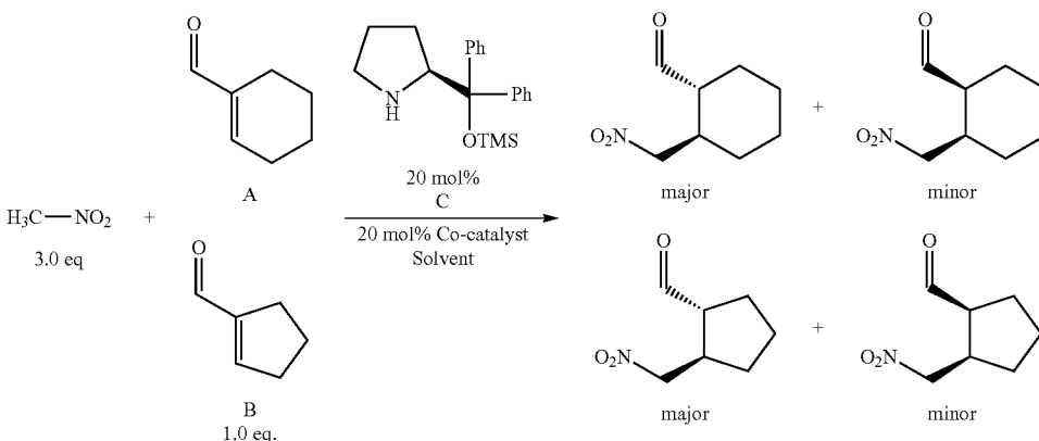
Scheme 5-A. Michael addition of nitromethane to cyclic enals.
