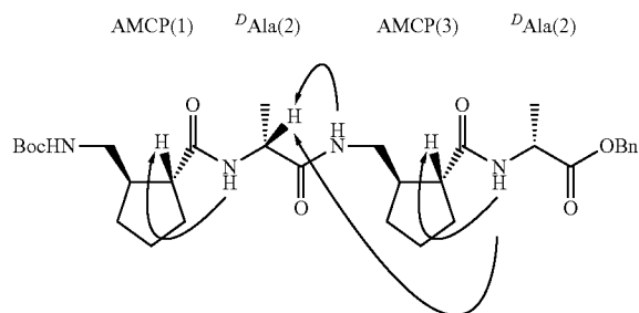
Scheme 5-5. A 1:1 α/γ-peptide tetramer (NOEs shown by arrows).
