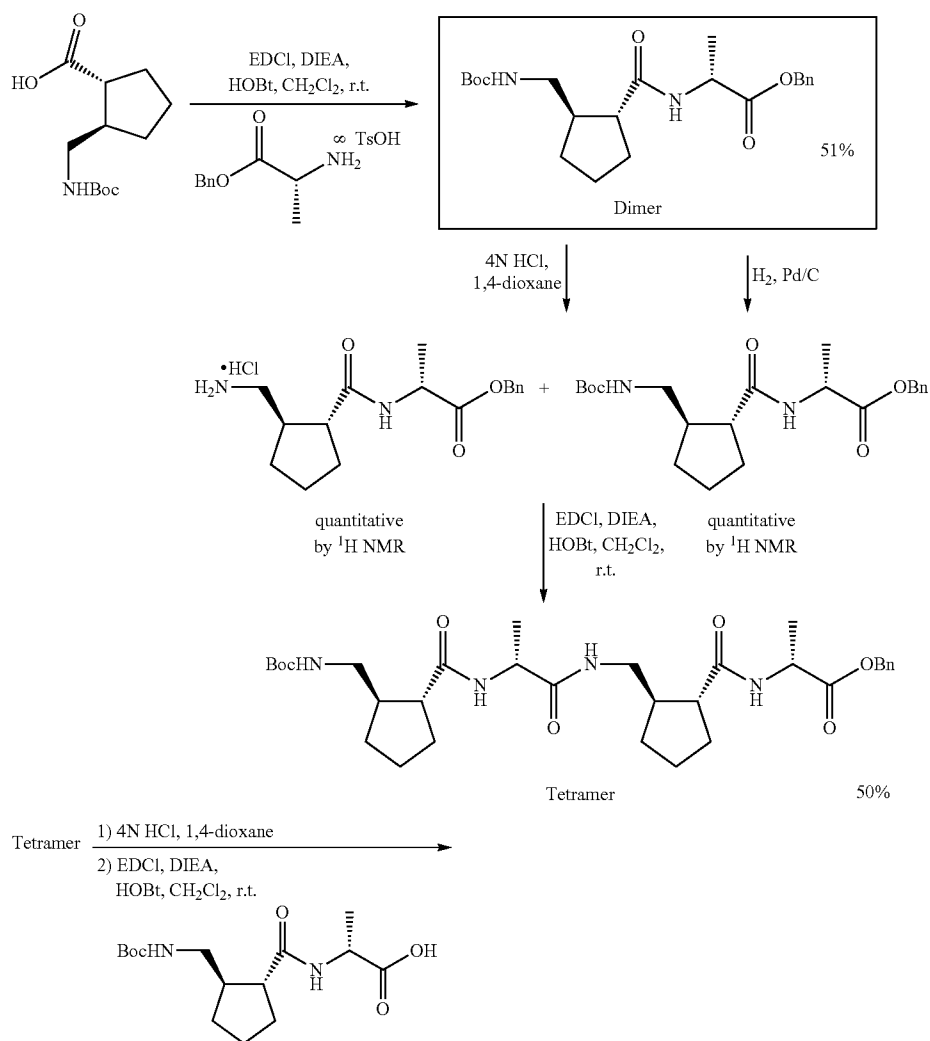
Scheme 5-4. Synthesis of 1:1 \alpha/\gamma -peptide oligomers.
