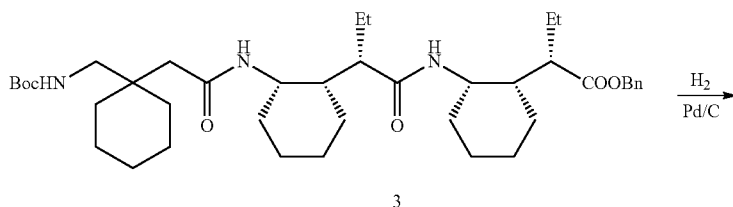
Scheme 7-5. Synthesis of oligomers 4-7.
