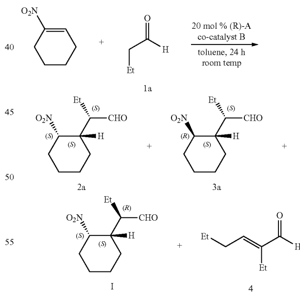
Scheme 1-1. Determination of d.r. of a Michael product by ^1H NMR assay
