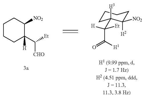
Scheme 1-3. 1 H NMR analysis of isolated product 3a
