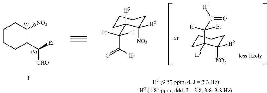
Scheme 1-4. 1 H NMR of isolated product I.
