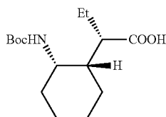
(S)-2-((1S,2S)-2-(tert-butoxycarbonylamino)cyclohexyl)butanoic acid
