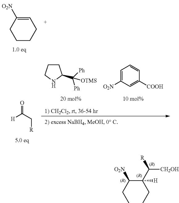
Scheme 2-1.
