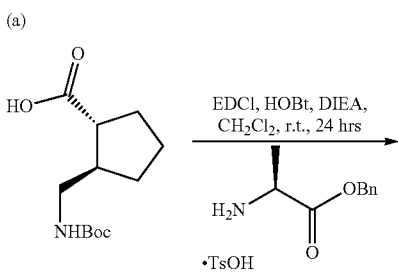
Scheme 5-3.
