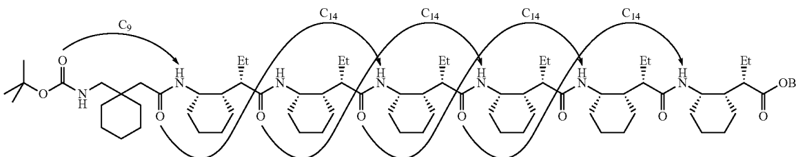
Scheme 8-5. \gamma -Peptides -14 Helix.
