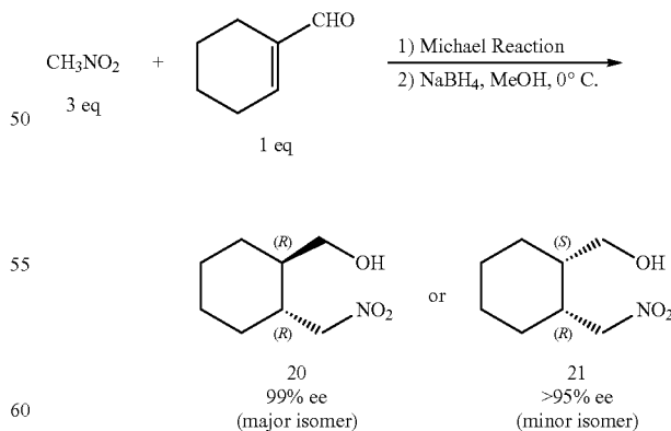
Scheme 4-1.
