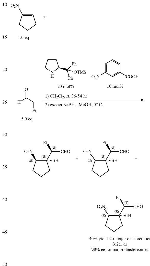
Scheme 2-2.
