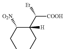
(S)-2-((1S,2S)-2-Nitrocyclohexyl)butanoic acid
