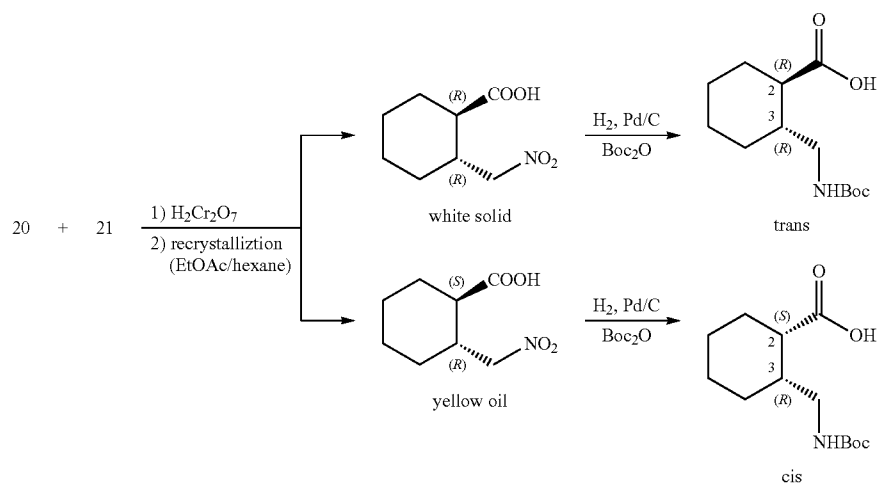
Scheme 4-2.
