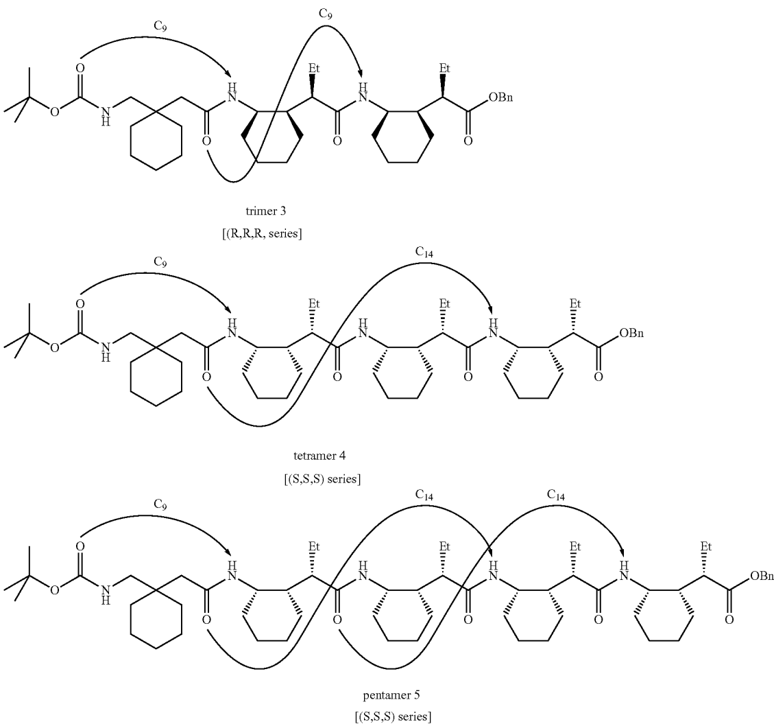
Scheme 7-6. Trimer 3, tetramer 4, and pentamer (S,S,S)-5.
