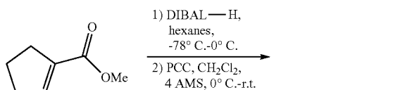
Scheme 5-2. Synthesis of 2-(Aminomethyl)-1-Cyclopentane Carboxylic Acid (AMCP) Building Blocks.
