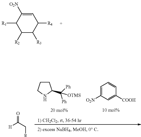
Scheme 3-1.
