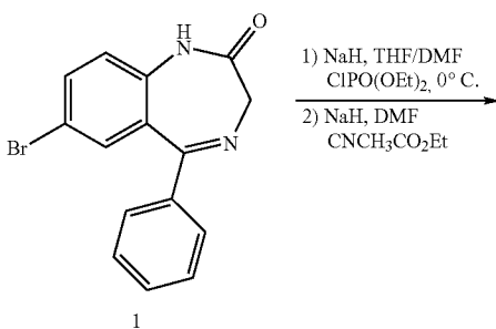
Scheme 8:
