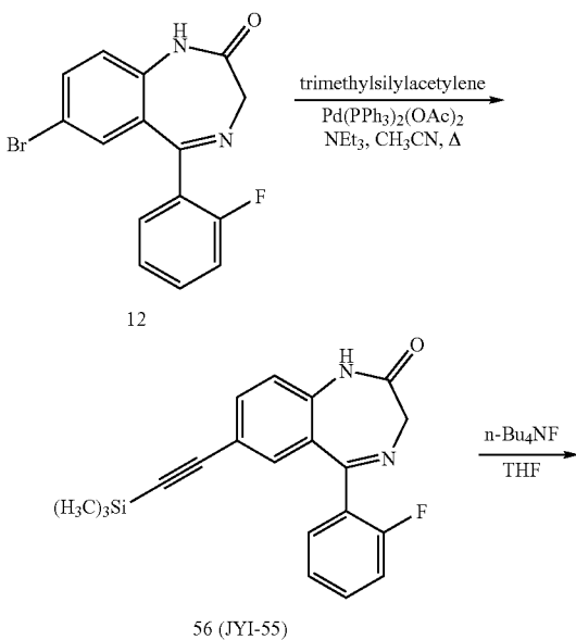
Scheme 12
