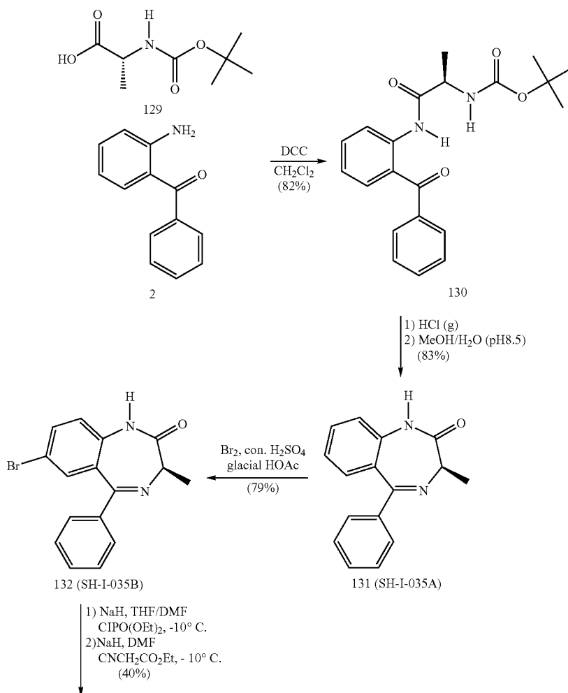
Scheme 26 (SH-053-R-CH 3 )
