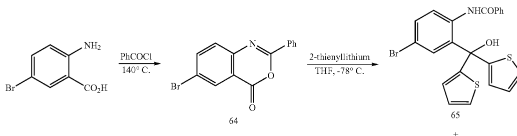
Scheme 14
