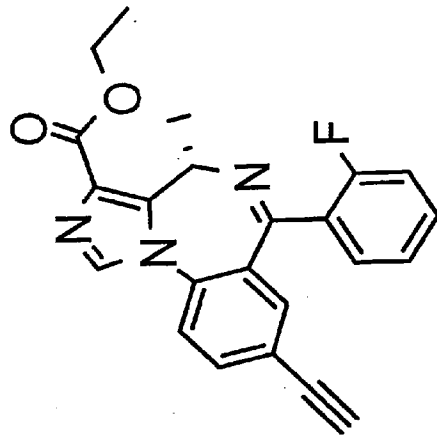
SH-053-2'F-S-CH3
