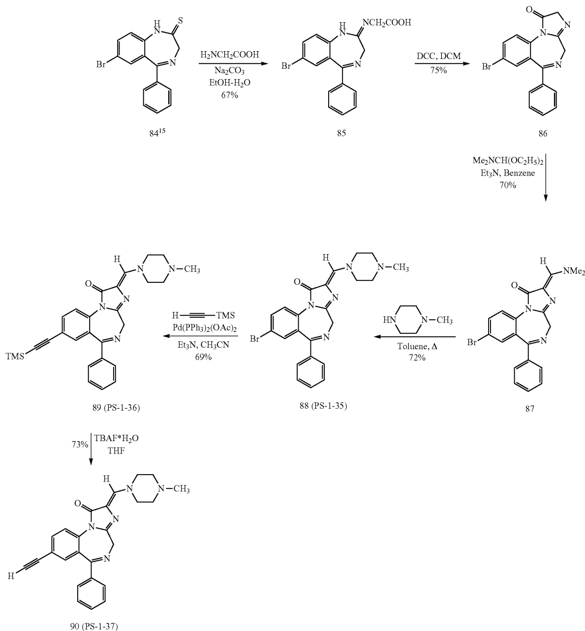
Scheme 17
