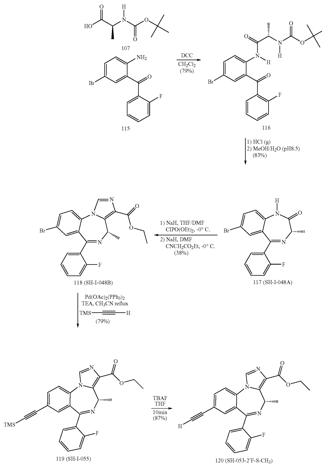
Scheme 24 (SH-053-2'F-S-CH 3 )
