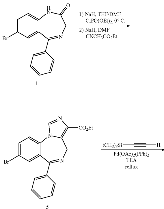
Scheme 2 (XHII-053)
