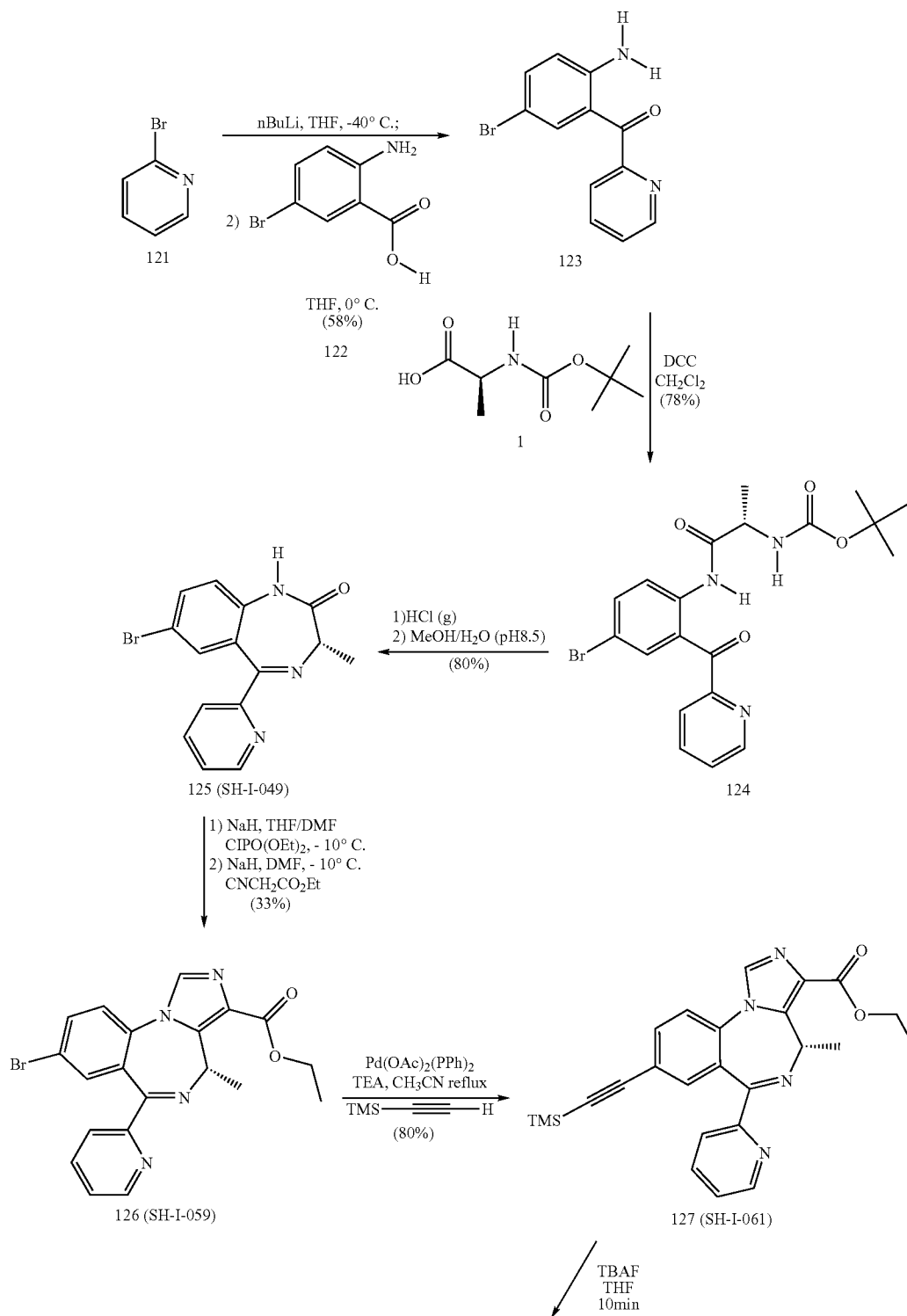
Scheme 25 (SH-053-2'N-S-CH 3 )
