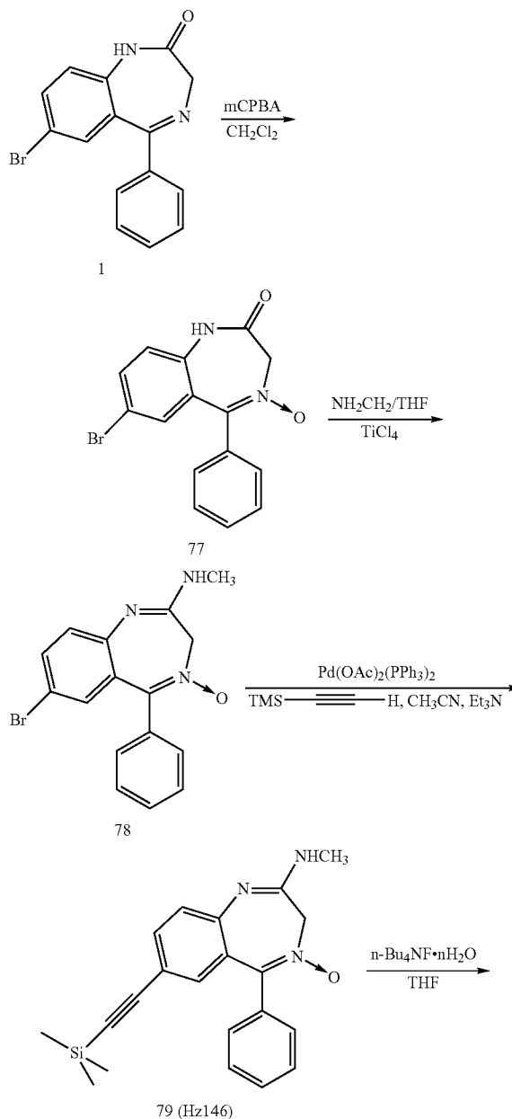
Scheme 15
