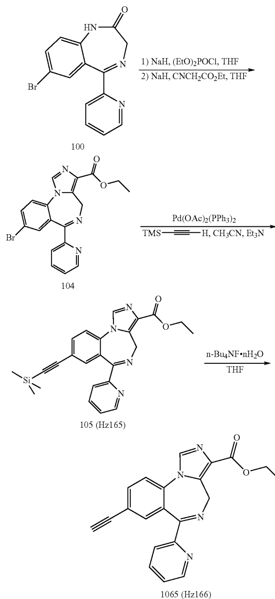
Scheme 22
