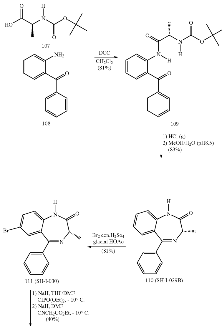
Scheme 23 (SH-053-S-CH 3 )
