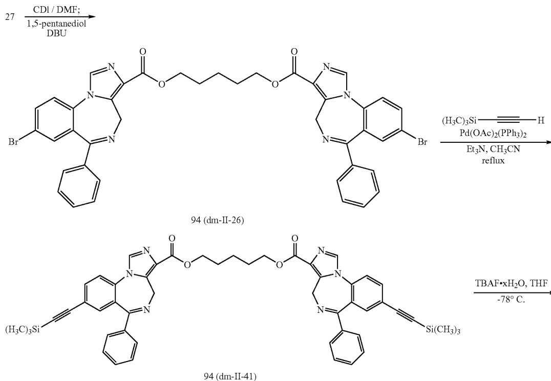
Scheme 19
